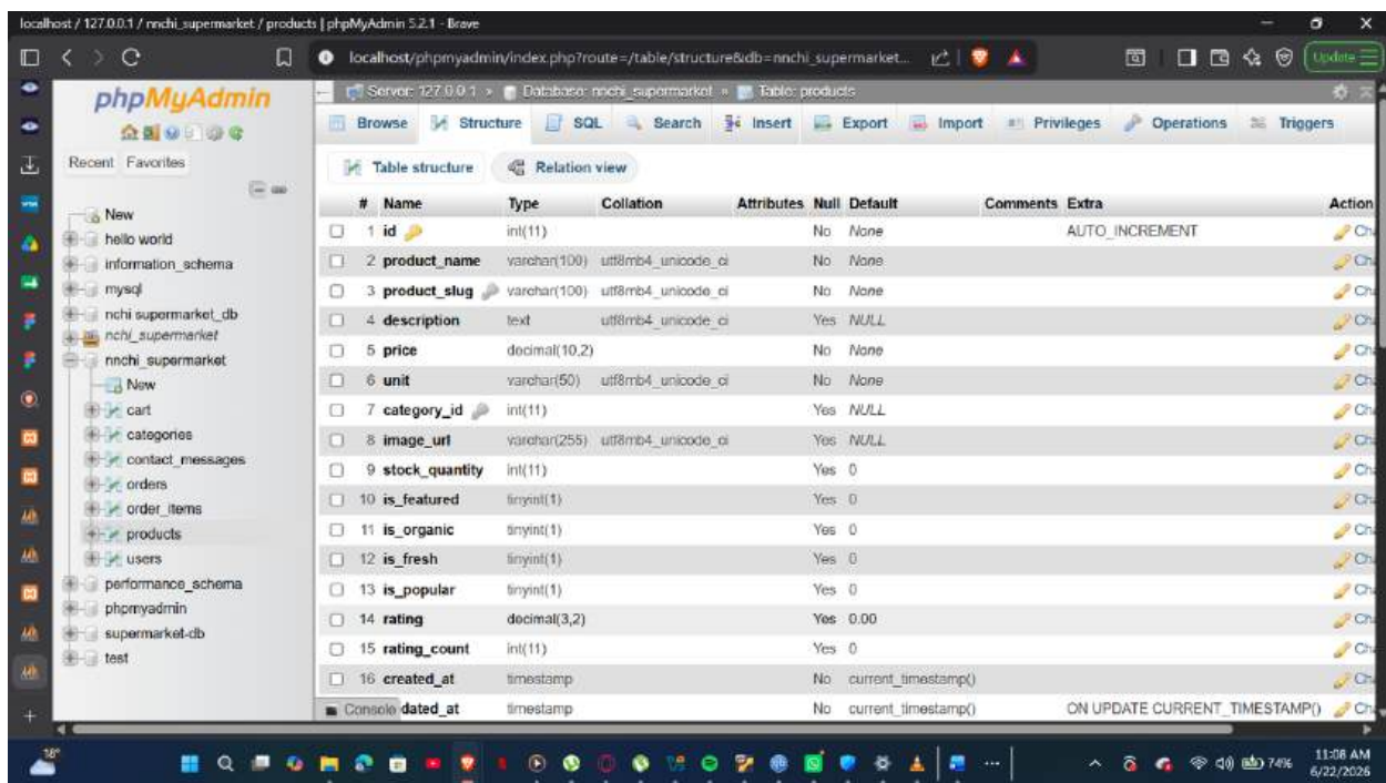
Fig 2 products table
