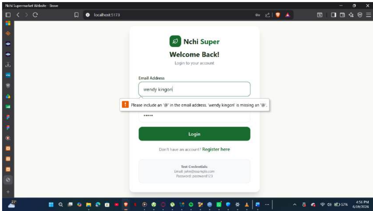
Fig 2 form validation
