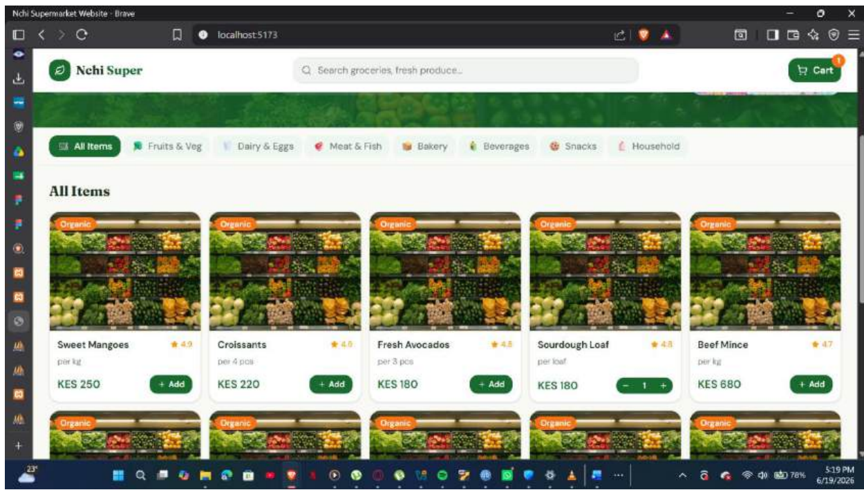
Fig 4 create
