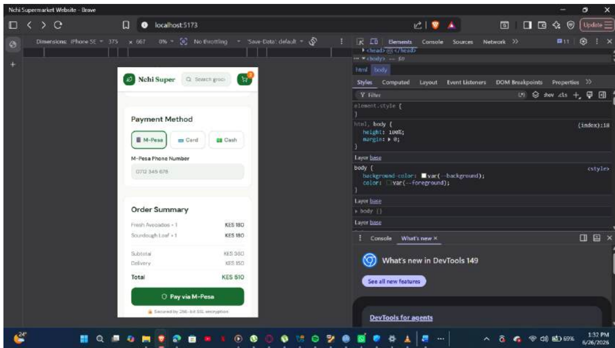
Fig 11checkout mobile.
