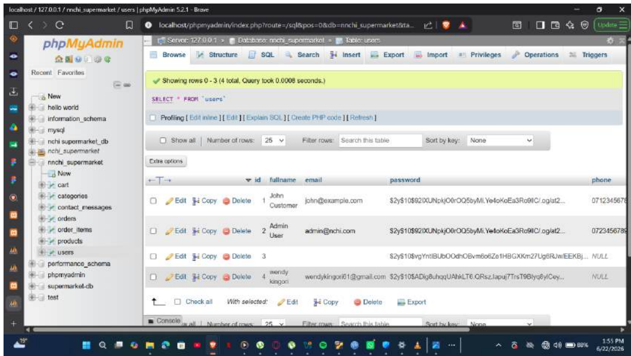
Fig 5 password hashing
