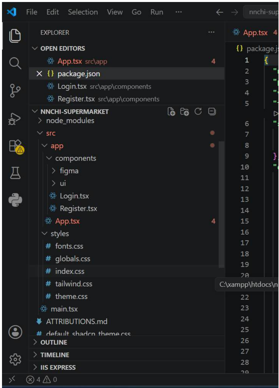
Fig 4 folder structure
