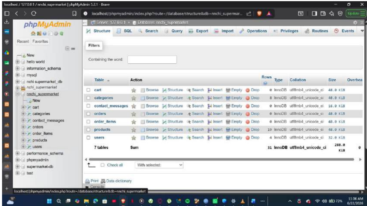
Fig 1 database
